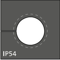
KTMB5 10-12 small (black), variable cable diameter range 10-12 mm
