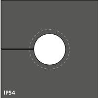
KTMB5 14-17 large (black), variable cable diameter range 14-17 mm
