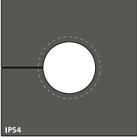
KTMB5 16-19 large (black), variable cable diameter range 16-19 mm
